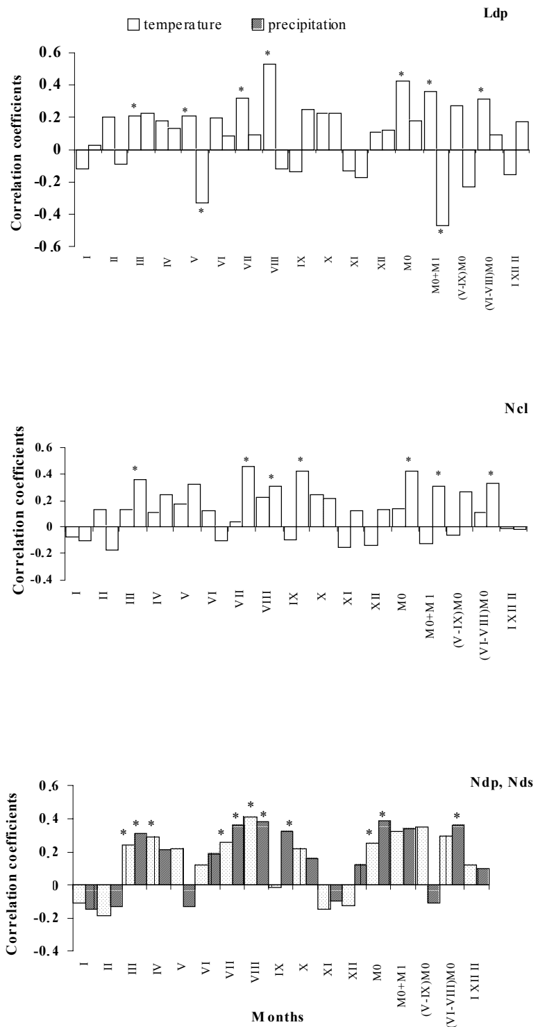
Fig. 3. Coefficients of correlation between the radial increment of oak stands and mean air temperatures (white bars) and precipitation sums (filled bars) over certain periods of time. The coefficients were calculated separately for temporarily overmoistured sites on very rich soils with coarse-on-fine soil texture (upper plot; site index Ldp), normally irrigated sites on rich, coarse-textured soils (Ncl) and for normally irrigated sites on very rich soils with fine and coarse-on-fine soil texture (Ndp; Nds). The arrows point at the coefficients that were significant at 0.05 level, where ( M_0 ) is the hydrological year (from past October to September of the next year); ( M_1 ) is the previous (earlier) hydrological year
