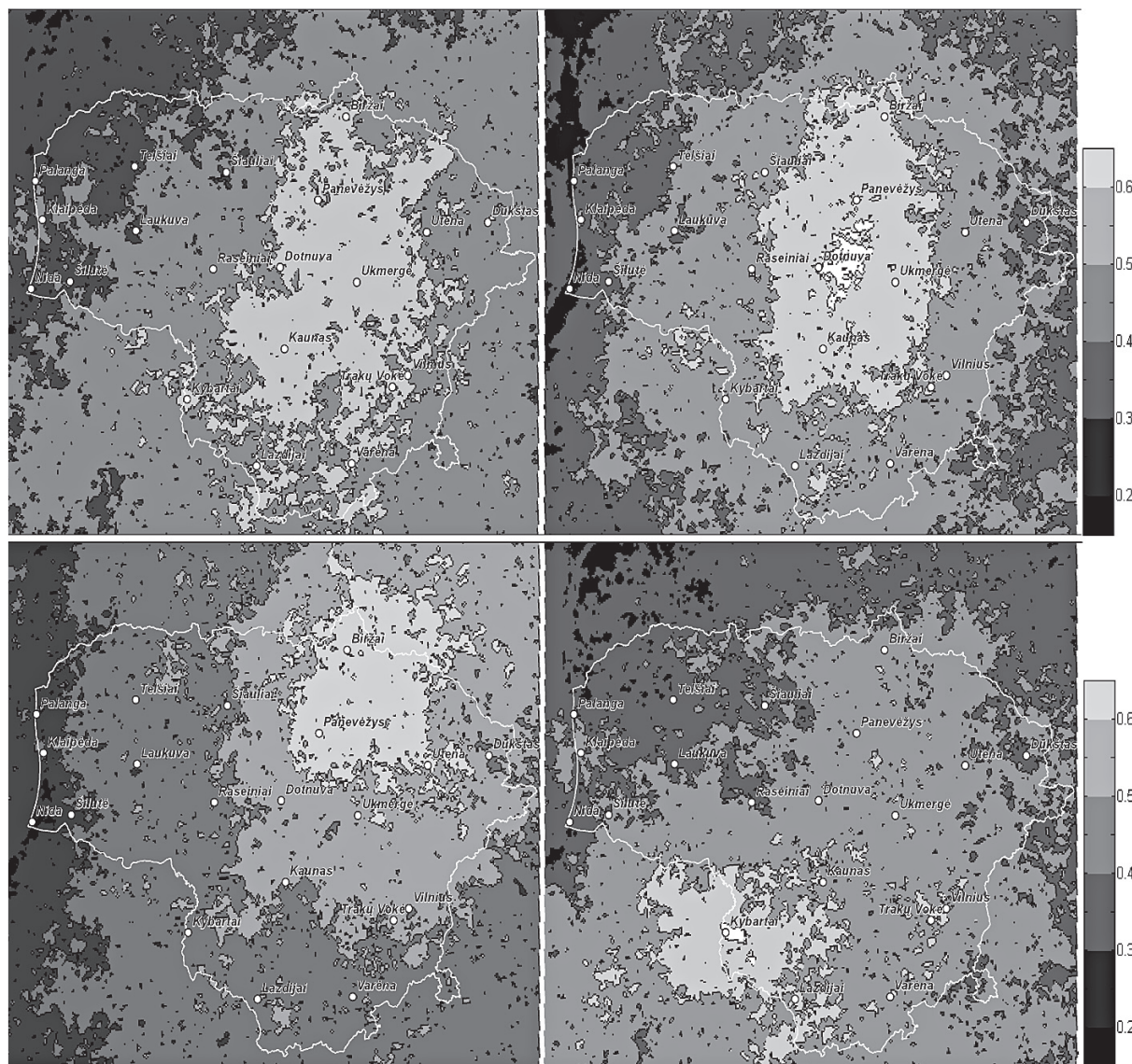
Fig. 4. The same as in Fig. 2, for Kaunas (upper left), Dotnuva (upper right), Biržai (lower left) and Kybartai (lower right) stations
