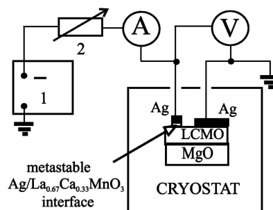
Fig. 2. Schematic diagram of the experimental set-up used for sample resistance measurements. 1 stabilized power source, 2 high-resistance potentiometer.
