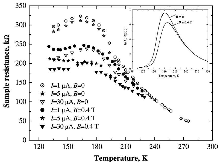
Fig. 7. Typical R - T plots of the \text{Ag}/\text{La}_{0.67}\text{Ca}_{0.33}\text{MnO}_3 interface in a metastable state corresponding to different current values; B = 0 and 0.4 T. Inset shows R - T plots of the \text{La}_{0.67}\text{Ca}_{0.33}\text{MnO}_3 film.
