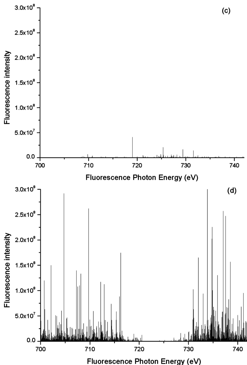
Fig. 1 (continued). Electric dipole 3s \rightarrow 2p and quadrupole 3p \rightarrow 2p emission in Co: (c) quadrupole transitions in CI approximation, (d) dipole transitions in the energy interval of quadrupole spectrum (relativistic CI approximation). The energy scales of all theoretical spectra are shifted to make the position of the main dipole maximum coincide with its observed position.
