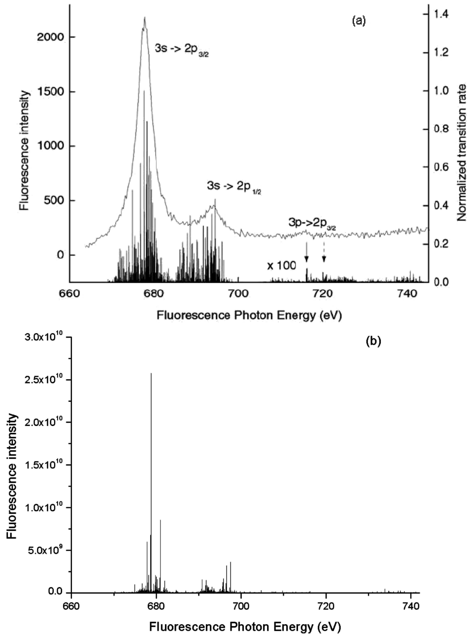
Fig. 1. Electric dipole 3s \rightarrow 2p and quadrupole 3p \rightarrow 2p emission in Co: (a) experiment and calculation in single configuration quasirelativistic approximation, reproduced with permission from [3], (b) calculation in relativistic CI approximation. The energy scales of all theoretical spectra are shifted to make the position of the main dipole maximum coincide with its observed position.
