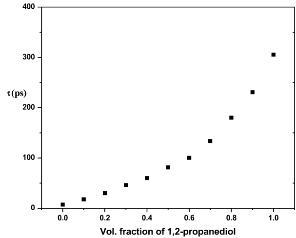
Fig. 5. Variation of relaxation time for 1,2-propanediol with dioxane content at 25 °C.
