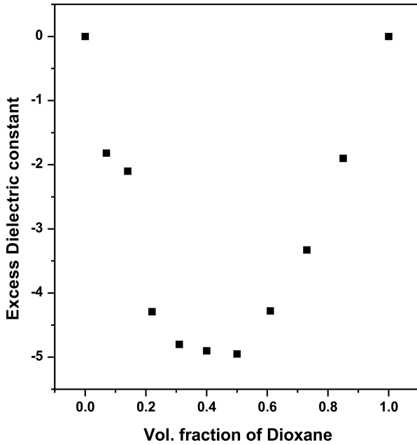
Fig. 6. Variation of excess dielectric constant for 1,2-propanediol with dioxane content at 25 °C.
