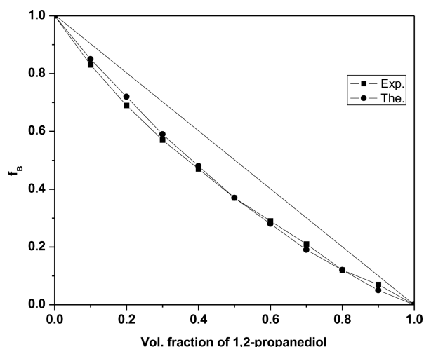
Fig. 9. Variation of Bruggeman dielectric factor with volume fraction of 1,2-propanediol in dioxane at 25 °C.
