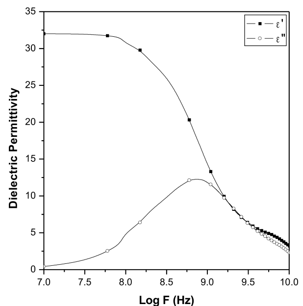
Fig. 2. Complex permittivity with frequency (GHz) at 25 °C.
