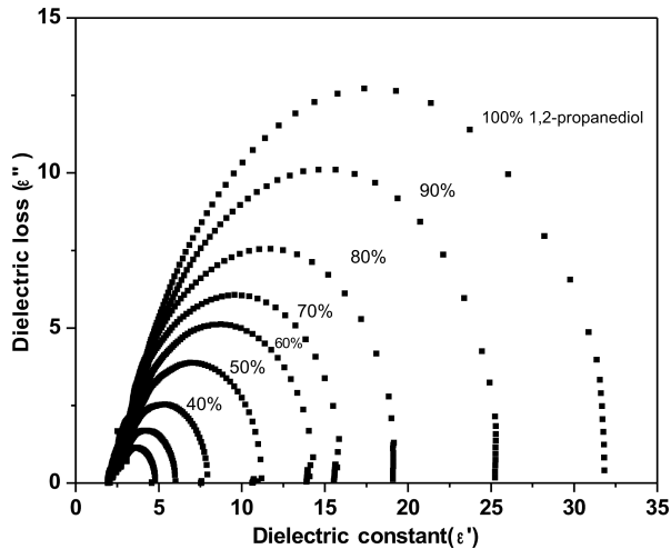
Fig. 3. Cole–Cole plot for 1,2-propanediol–dioxane mixtures at 25 °C.
