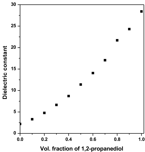
Fig. 4. Variation of static dielectric constant for 1,2-propanediol with dioxane content at 25 °C.
