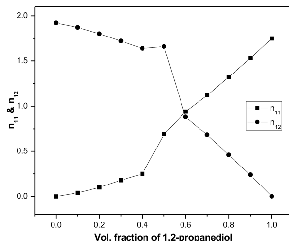
Fig. 8. Plot of average number of hydrogen bonds between 1,2-propanediol–1,2-propanediol molecules (11-pair) and 1,2-propanediol–dioxane (12-pair).
