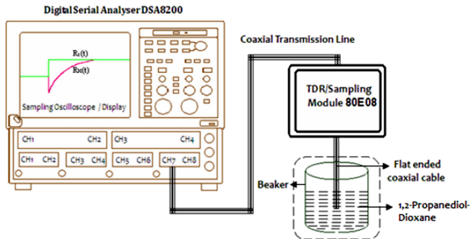
Fig. 1. Block diagram of time domain reflectometry (TDR).
