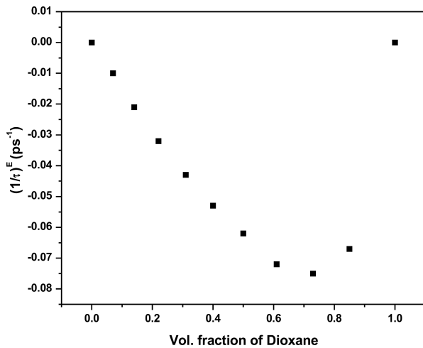
Fig. 7. Variation of inverse excess relaxation time for 1,2-propanediol with dioxane content at 25 °C.
