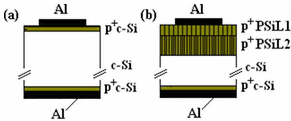
Fig. 1. Schematic drawings of two silicon structures with additionally boron-doped top and bottom: (a) crystalline silicon sample, (b) microporous silicon sample.
