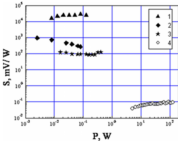
Fig. 3. Voltage sensitivity of the devices as a function of microwave power: 1, 2, 3 are \mu PSi containing samples; 4 is a reference c-Si sample. Sample resistance: 1 10 k \Omega , 2 4.2 k \Omega , 3 500 \Omega , 4 5 k \Omega .
