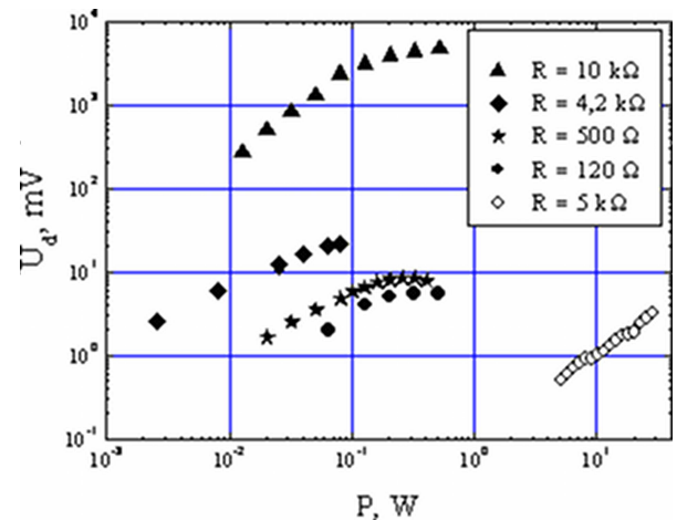
Fig. 2. Dependences of response amplitude on microwave power: open diamonds for c-Si device, other points for devices containing PSi layers.
