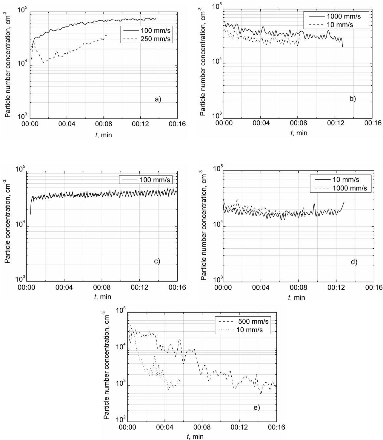
Fig. 4. Dynamics of generated particle number concentration during laser ablation of various metals in ambient air: (a) nickel by ns-laser at 0.4 W, 20 kHz, 1.59 J/cm 2 and (b) by ps-laser at 0.49 W, 100 kHz, 1.56 J/cm 2 ; (c) tungsten by ns-laser at 0.85 W, 22 kHz, 3.07 J/cm 2 and (d) by ps-laser at 0.25 W, 100 kHz, 1.80 J/cm 2 ; (e) aluminum by ns-laser at 0.6 W, 50 kHz, 3.82 J/cm 2 .
