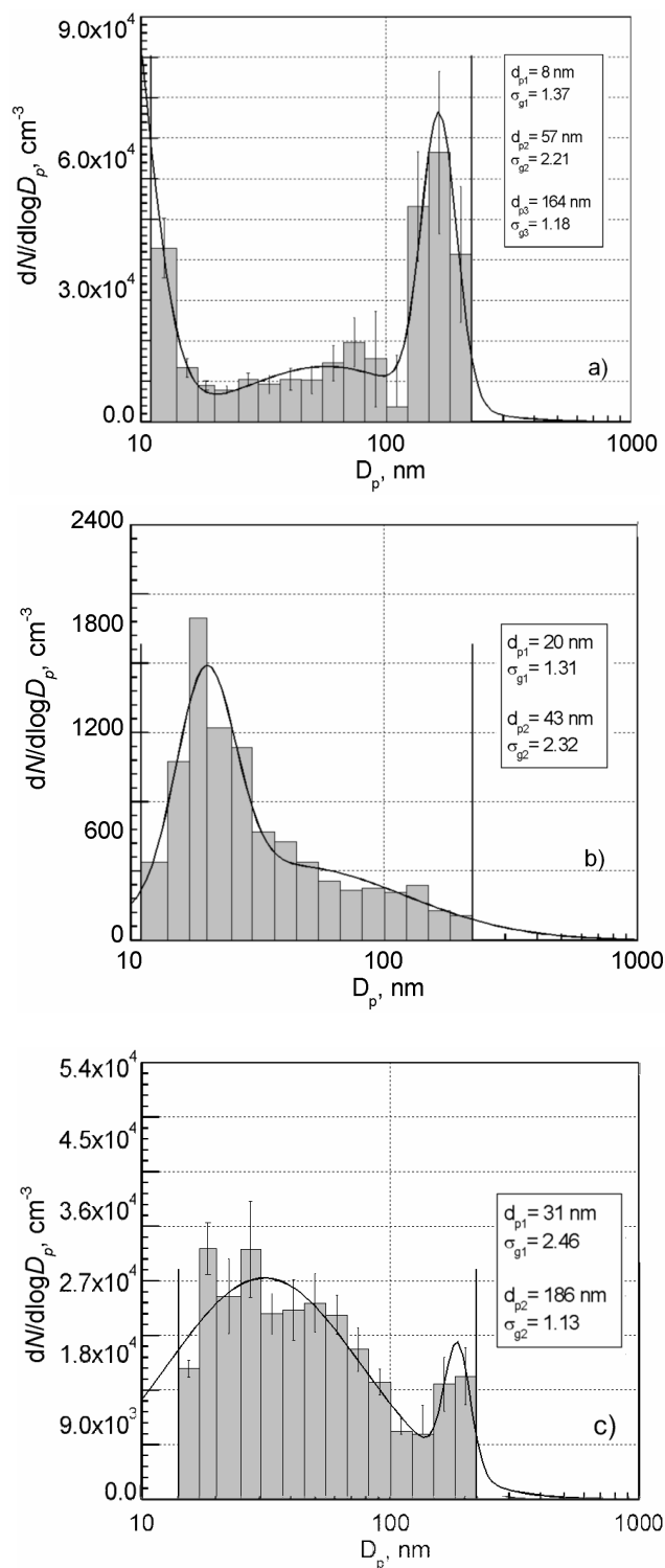
Fig. 3. Particle size D_p distribution for the ps-laser ablation in ambient air: (a) nickel at 0.25 W, 100 kHz, 10 mm/s and 0.80 J/cm 2 ; (b) aluminum at 0.6 W, 50 kHz, 10 mm/s and 3.82 J/cm 2 ; (c) tungsten at 0.25 W, 100 kHz, 1 000 mm/s and 0.80 J/cm 2 .
