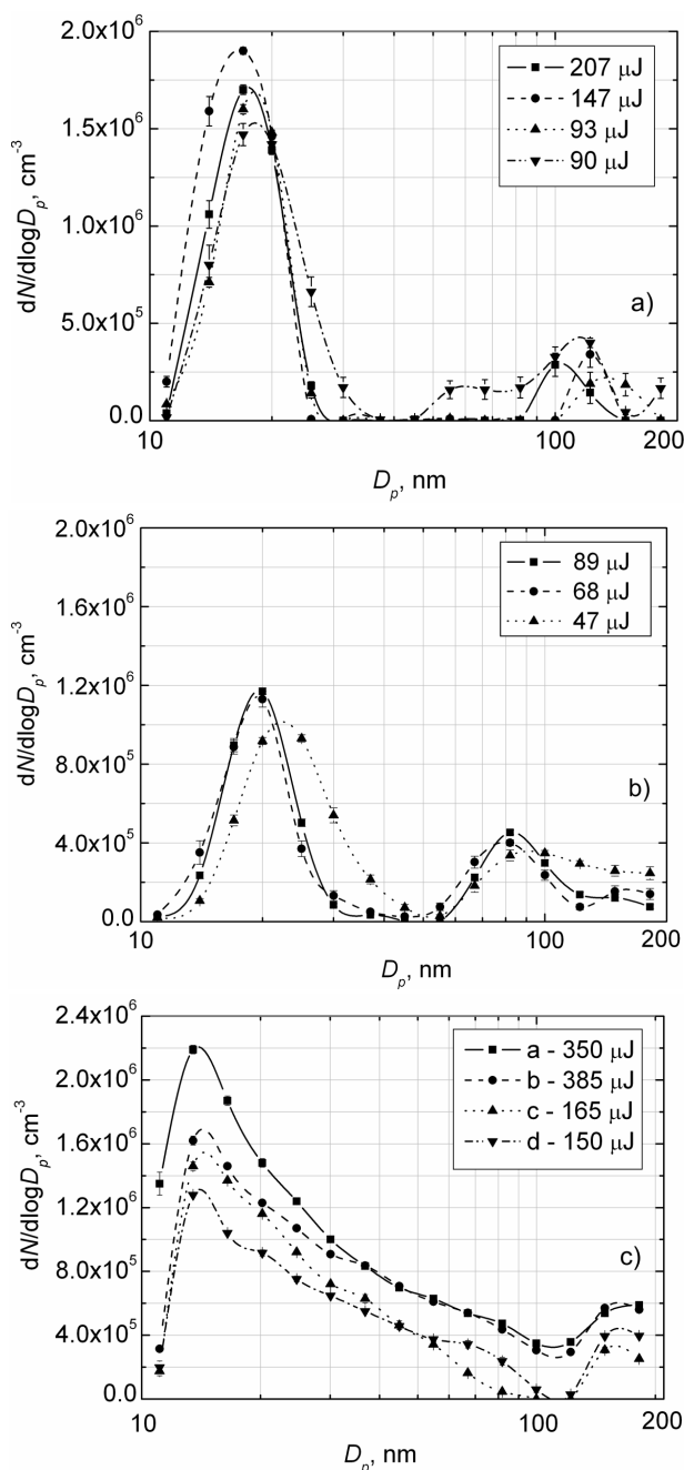
Fig. 6. Particle size d_p distribution for ns-laser ablation of metals in argon gas at different beam intensities: (a) nickel at 10–30 kHz, 10–100 mm/s (16.47, 11.70, 7.40 and 7.16 J/cm 2 respectively to the laser pulse energy); (b) aluminum at 10–20 kHz, 100–500 mm/s (7.08, 5.41 and 3.74 J/cm 2 respectively to the laser pulse energy) and (c) stainless steel at 1–20 kHz, 10–100 mm/s (27.85, 30.64, 13.13 and 11.94 J/cm 2 respectively to the laser pulse energy).
