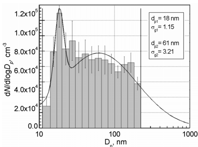
Fig. 2. Particle size ( D_p ) distribution for the ns-laser ablation of nickel in ambient air at 0.4 W, 10 kHz, 200 mm/s and 12.73 J/cm 2 .
