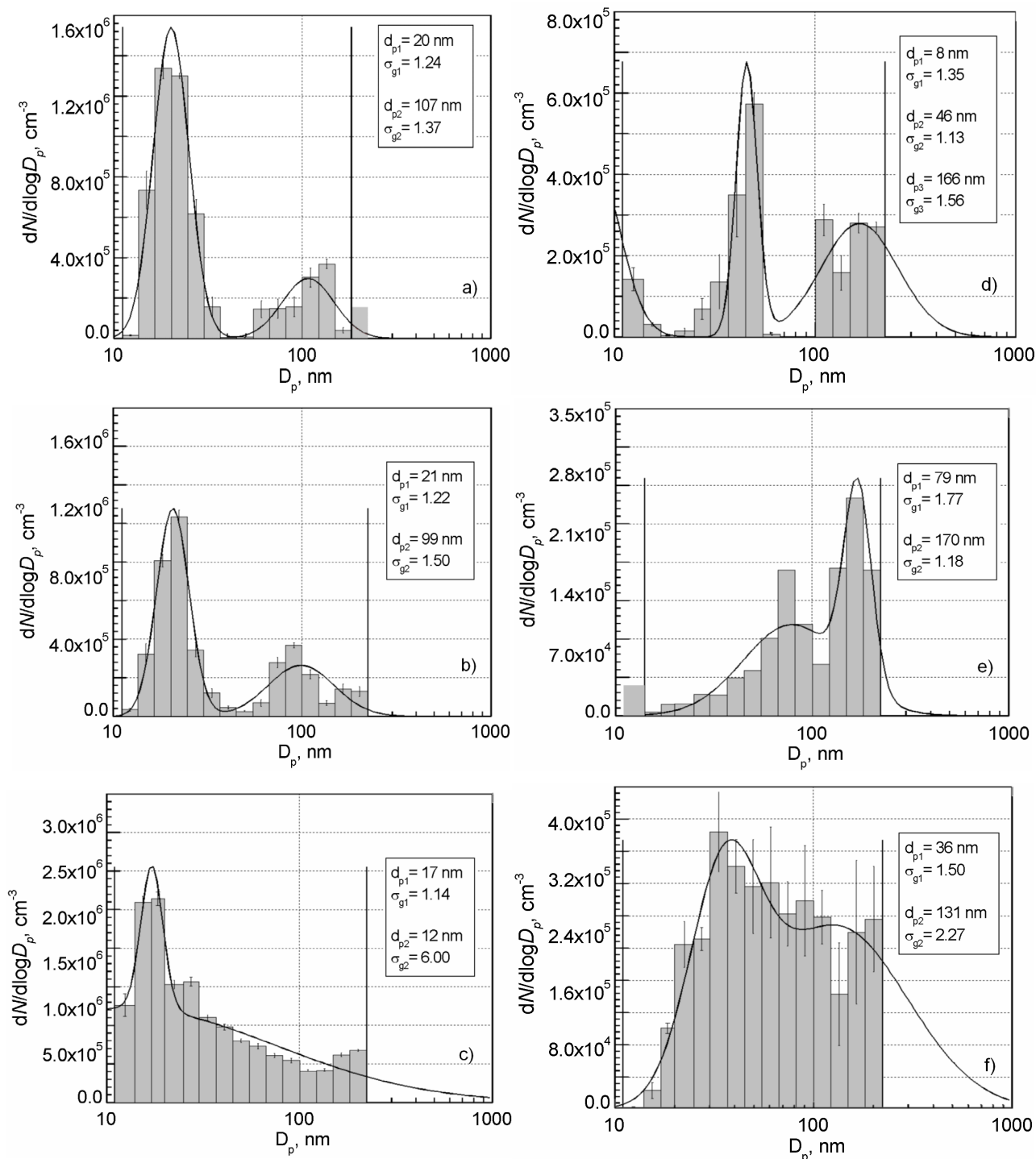
Fig. 5. Particle size d_p distribution for the ns-laser ablation of various metals in argon gas: (a) nickel at 2.7 W, 30 kHz, 10 mm/s, 7.16 J/cm 2 ; (b) aluminum at 1.36 W, 20 kHz, 100 mm/s, 5.41 J/cm 2 ; (c) stainless steel at 1.75 W, 5 kHz, 10 mm/s, 27.85 J/cm 2 and the ps-laser ablation in argon gas: (d) nickel at 1.5 W, 50 kHz, 100 mm/s, 9.55 J/cm 2 ; (e) aluminum at 0.6 W, 50 kHz, 100 mm/s, 3.82 J/cm 2 ; (f) tungsten at 1.2 W, 100 kHz, 100 mm/s, 3.82 J/cm 2 .
