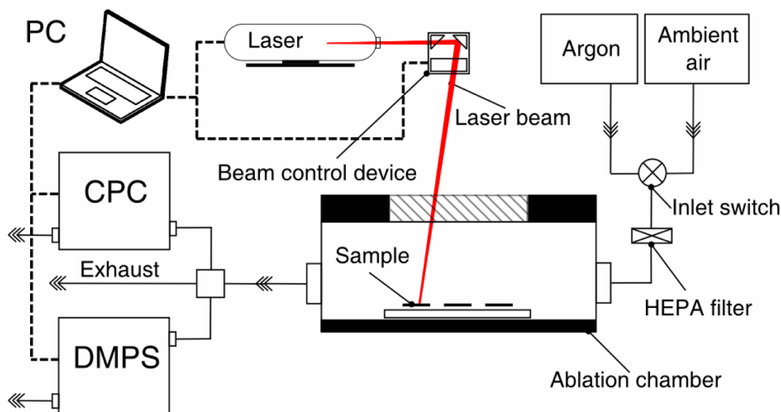
Fig. 1. Experimental set-up for generated particle measurement.
